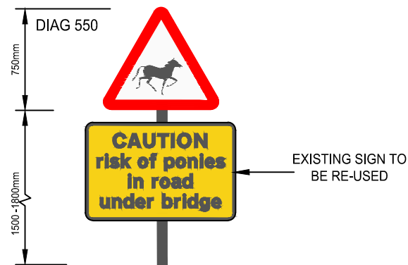
ASSEMBLY 'D'
