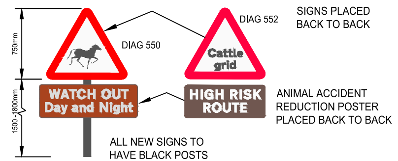
ASSEMBLY 'E'
